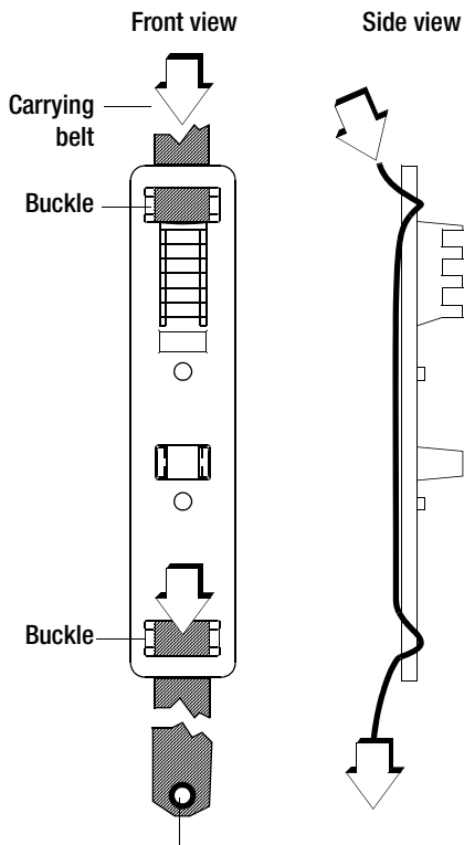
Fastening eye for (METRISO ...) test instrument
