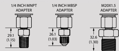
ADDITIONAL SENSOR LENGTH WITH OPTIONAL FITTING ADAPTERS
