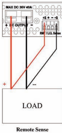
Remote Sense
