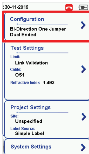
[SETUP]
