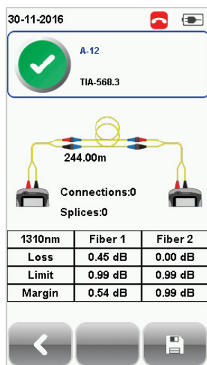
SingleMode 1310 nm
