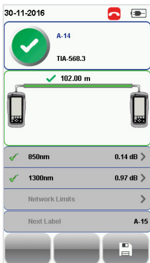
Multimode
