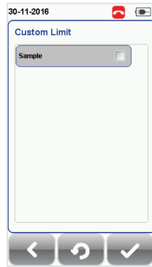
Custom Limit
