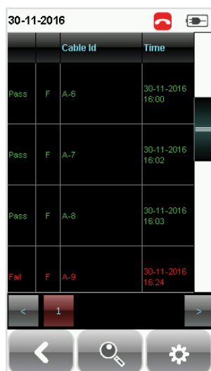
View results
