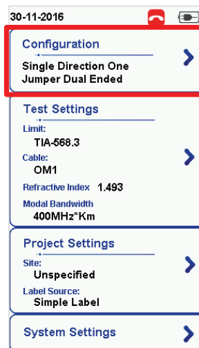
[SETUP]
