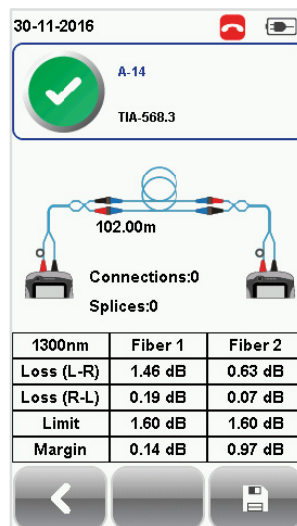
Multimode 1300 nm
