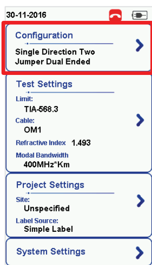
[SETUP]
