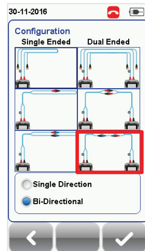
Multimode [Configuration]
