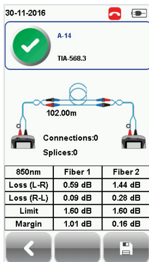
Multimode 850 nm
