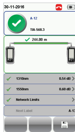
AUTOTEST complete
