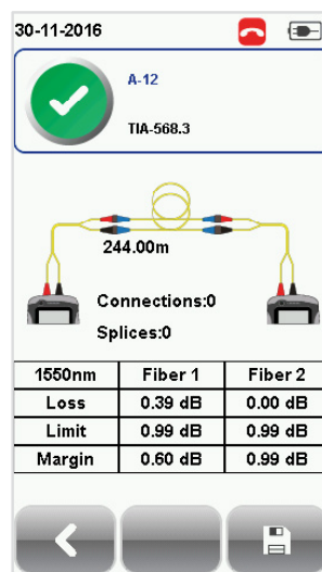
SingleMode 1550 nm
