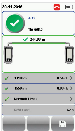
SingleMode
