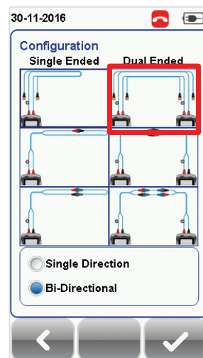
Multimode [Configuration]
