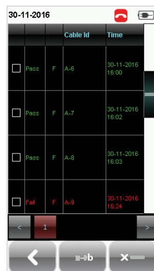
Manage results
