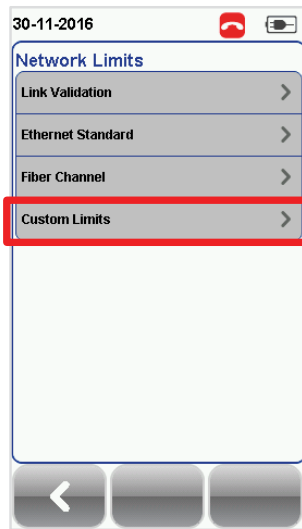
Network Limits
