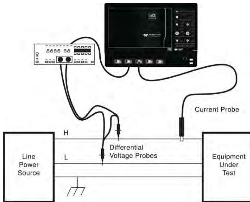
Typical line power analysis circuit setup
