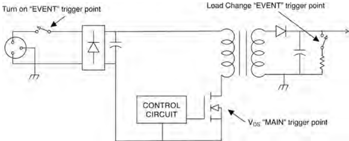
Typical trigger points for device analysis.
