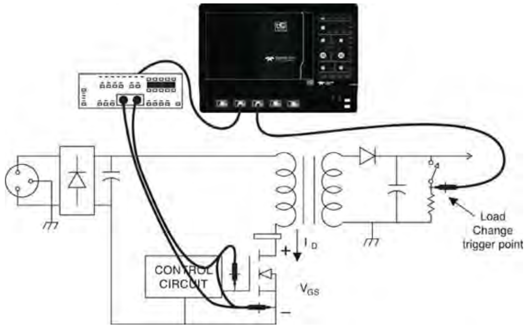
Typical control loop analysis circuit setup
