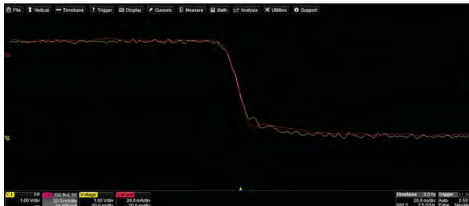
Falling edge of voltage and current traces after deskew adjustment.
