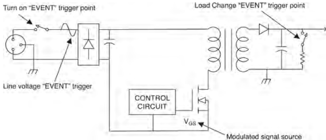
Typical control loop analysis triggers
