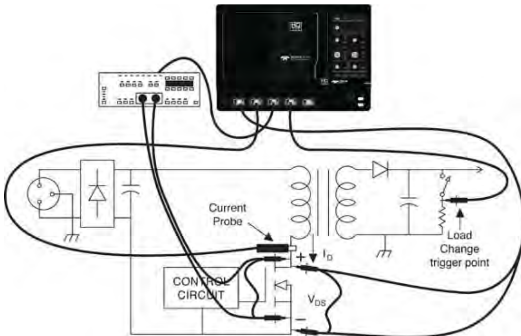
Typical probing points for device analysis.
