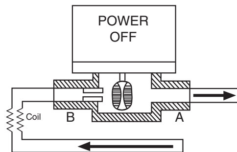
Figure-6b 2-Way Valve With Normally Open Actuator
