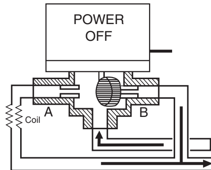
Figure-6f 3-Way Valve in Diverting Configuration Normally Open to the Coil
