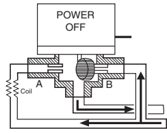
Figure-3d 3-Way Valve in Mixing Configuration Normally Open to the Coil.
