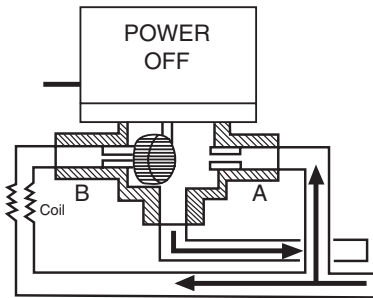
3-Way Valve in Mixing Configuration, Normally Closed to the Coil
