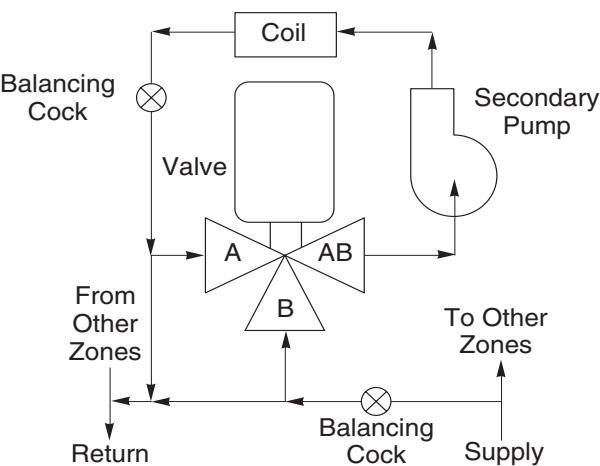
Figure 8. Typical Primary-Secondary Piping
