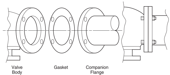
Figure 5. Installation of Flanged End Valves.
