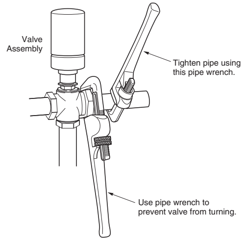
Figure 4. Installation of Screwed End Valves.
