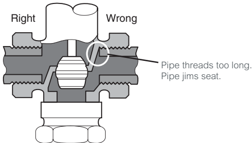
Figure 3. Normal Thread Engagement.
