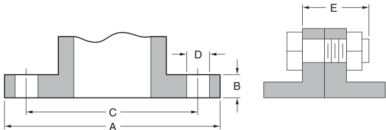
Figure 11. Flange Dimensions.
