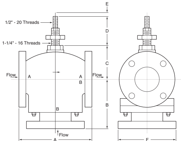
Figure 10. Typical of VB-9313-0-5-P, 2½"...6" Valve Bodies.
