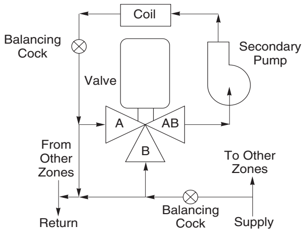
Figure 8. Typical Primary-Secondary Piping
