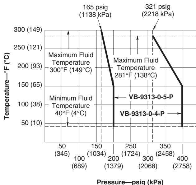
Figure 2. Temperature and Pressure Ratings for VB-9313 Series Valve Bodies.
