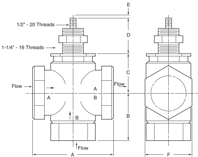
Figure 9. Typical of VB-9313-0-4-P, 2½" and 3" Valve Bodies.
