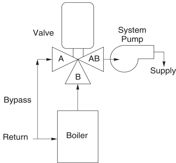
Figure 7. Typical Boiler Hot Water Reset
