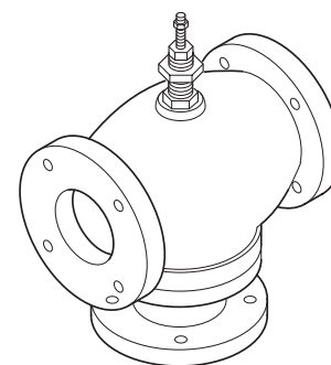
Typical of VB-9313-0-5-P 2½" to 6"
