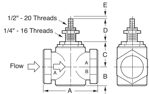
Figure-6 Typical of VB-9213-0-4-P, 2-1/2" and 3" Valve Bodies.
