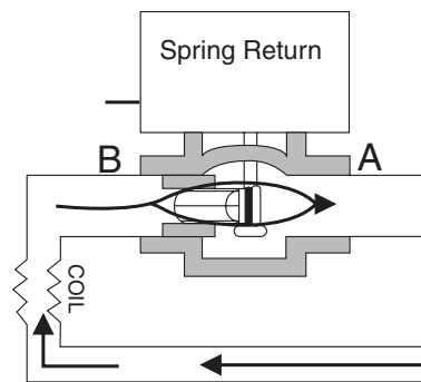
Figure 2 Two-Way Valve Normally Open.
