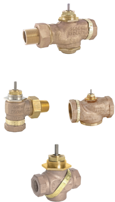
Venta VB-7200 Series 2-way globe valves
