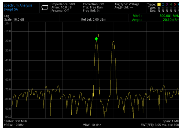
Figure 3-7 Distinguished Two Equal-Amplitude Signal (2)
