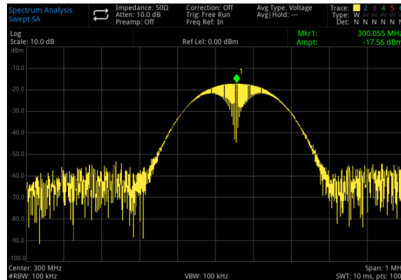
Figure 3-5 Undistinguished Two Equal-Amplitude Signals
