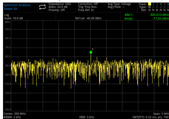
Figure 3-13 Reduce Resolution Bandwidth
