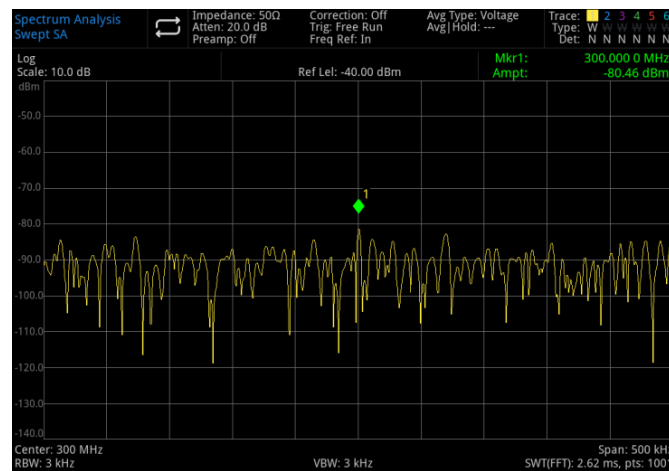
Figure 3-11 A Signal Close to Ground Noise
