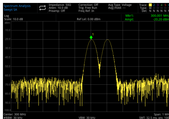
Figure 3-6 Distinguished Two Equal-Amplitude Signal (1)
