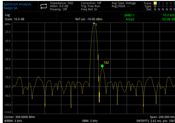
Figure 3-9: Distinguish Small Signal from Big Signal
