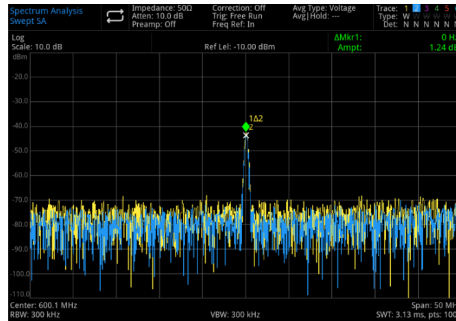
Figure 3-17 Component of Harmonic Distortion
