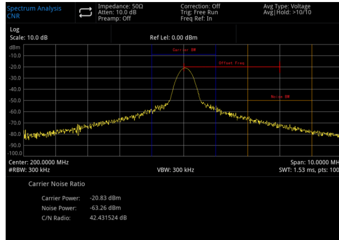
Figure 5-7 Measurement of Carrier-to-Noise Ratio
