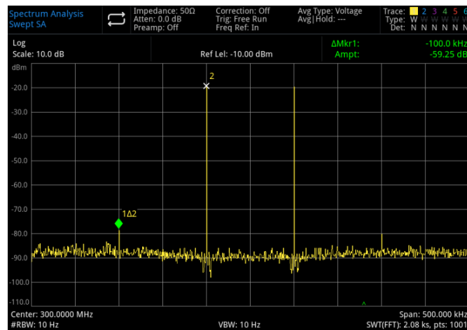
Figure 3-19 Measuring Distortion Product
