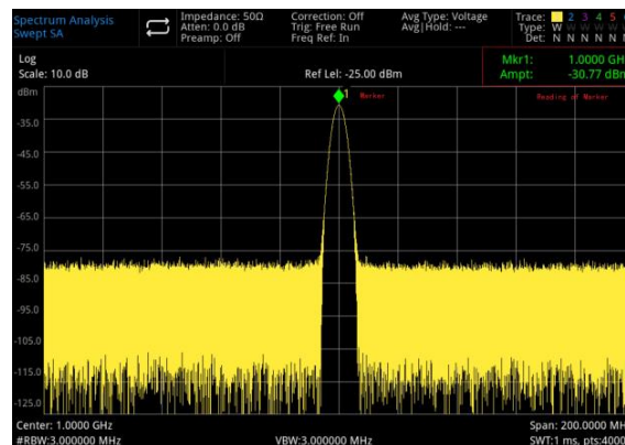
Figure 4-1 Reading of Marker Cursor
