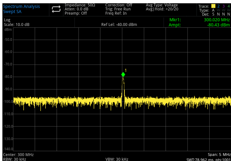
Figure 3-14 Trace Averaging
