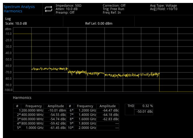
Figure 5-8 Harmonic Measurement
