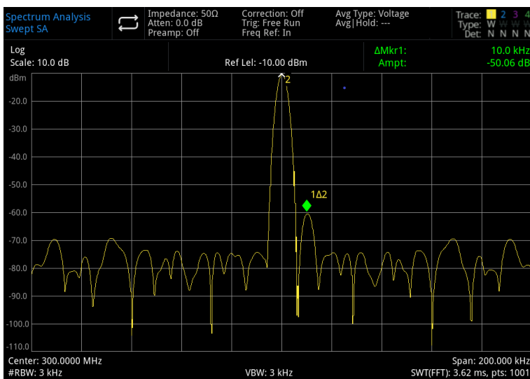
Figure 3-9: Distinguish Small Signal from Big Signal
