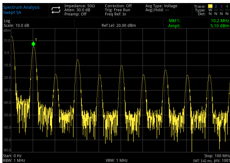
Figure 3-1 Read Frequency and Amplitude
