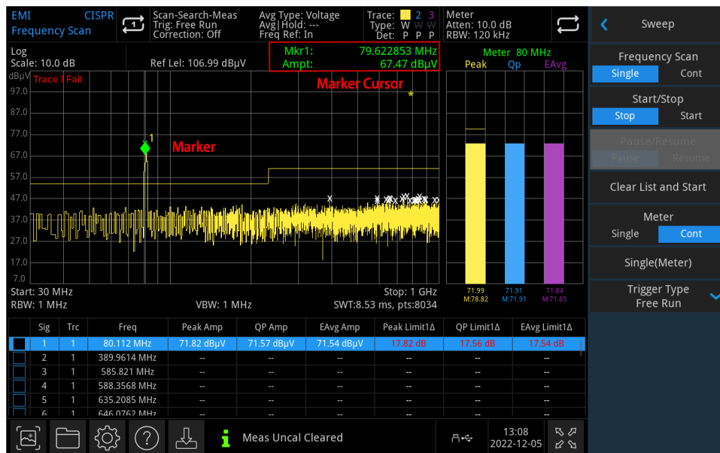
Figure 3-1 Reading of Marker Cursor
