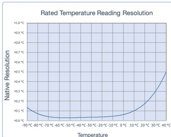
Figure 5: Rated Temperature Resolution Chart
