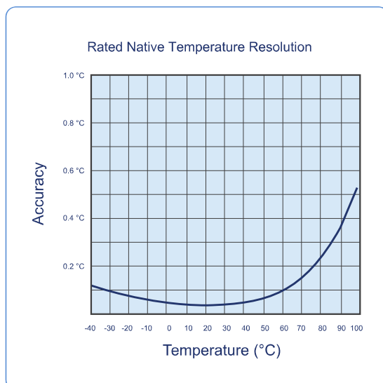
Figure 5: Rated Temperature Resolution Chart
