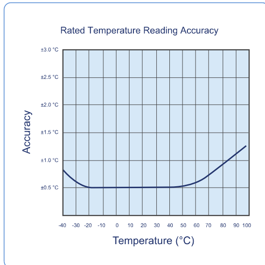
Figure 4: Rated Temperature Accuracy Chart
