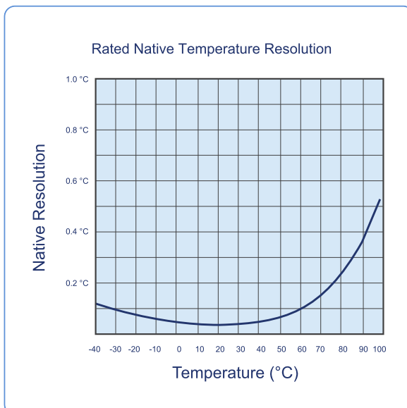
Figure 10: Rated Temperature Resolution Chart
