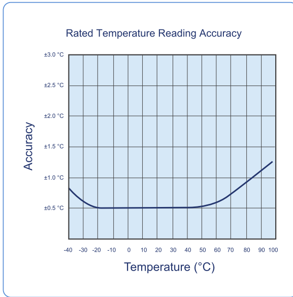
Figure 9: Rated Temperature Accuracy Chart
