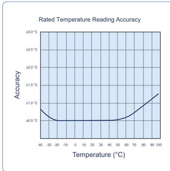
Figure 6: Rated Temperature Accuracy Chart
