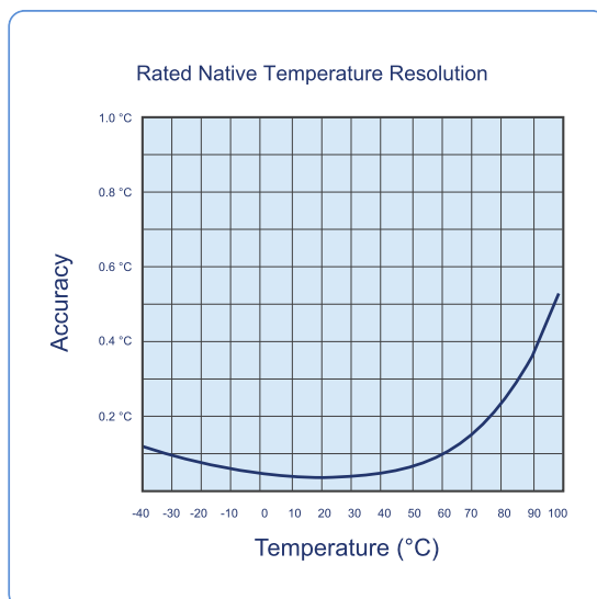
Figure 7: Rated Temperature Resolution Chart
