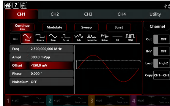
Figure 2-6 DC Offset Voltage Settings
