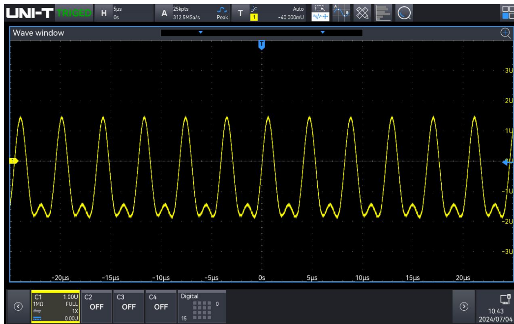
Sine with harmonic distortion
