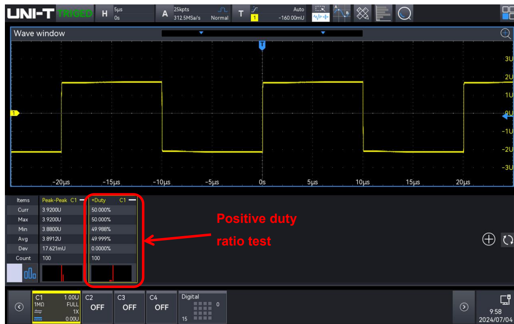
Demo result of square wave
