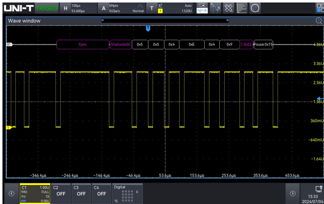
SENT trigger and decoding
