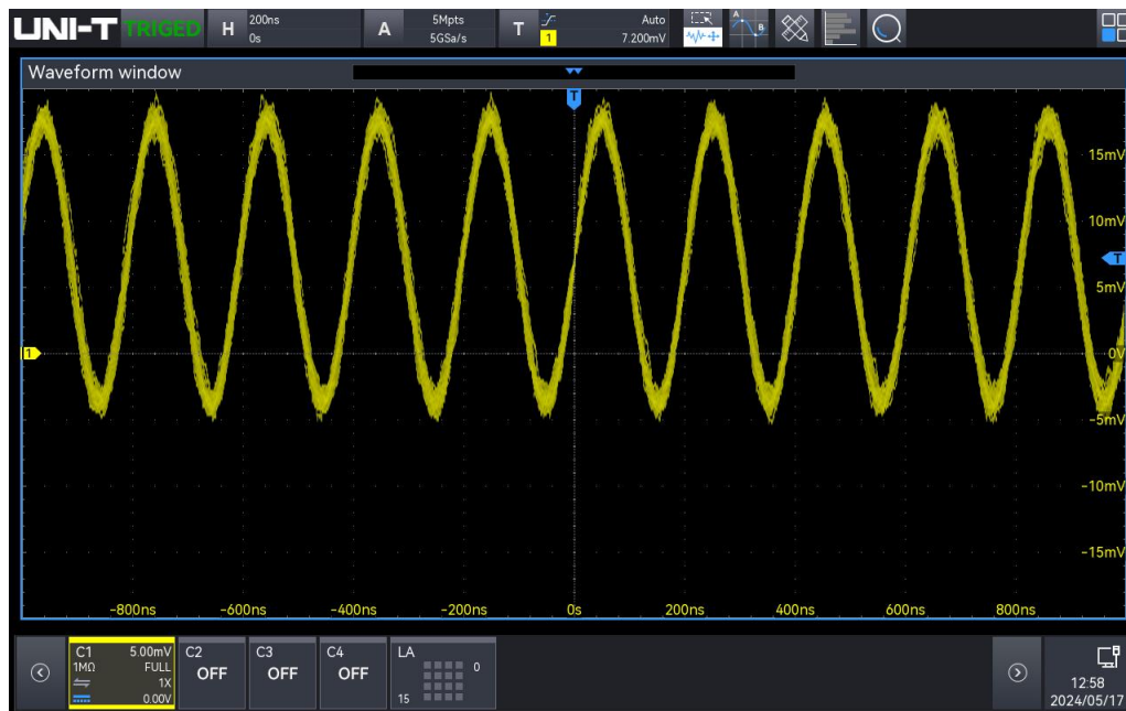
Clock with jitter
