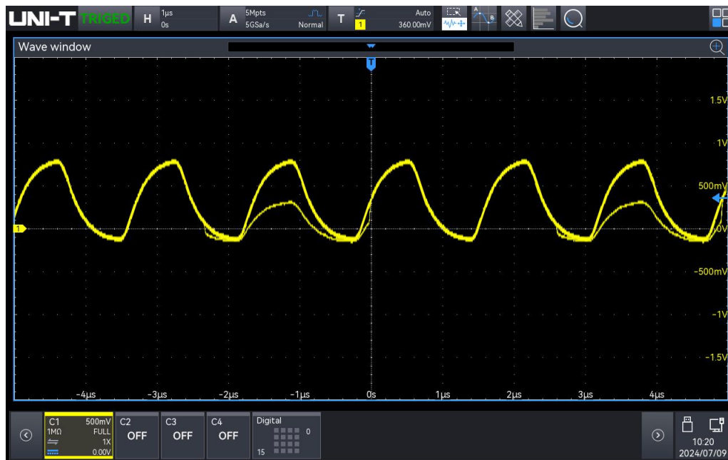
Clock with infrequent glitch
