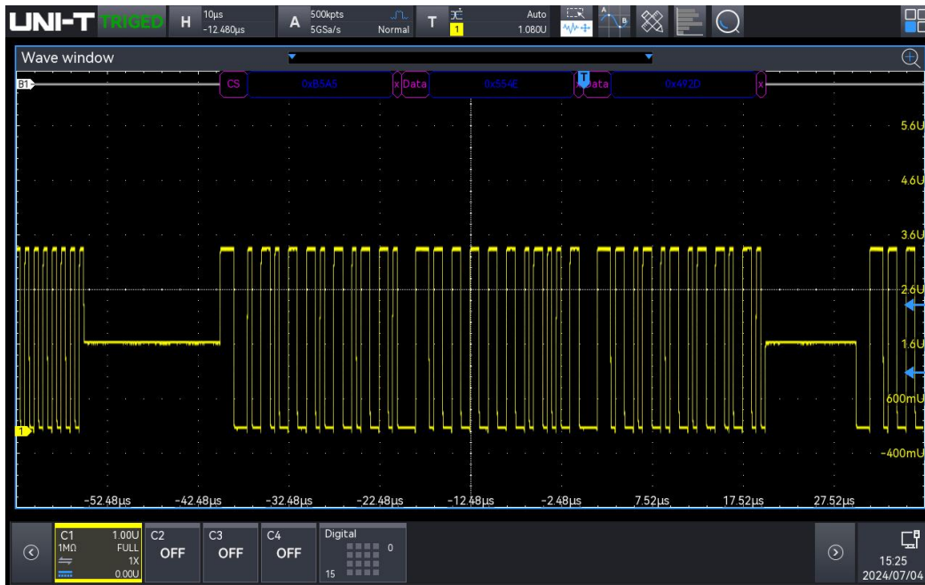
1553B data block trigger and decoding
