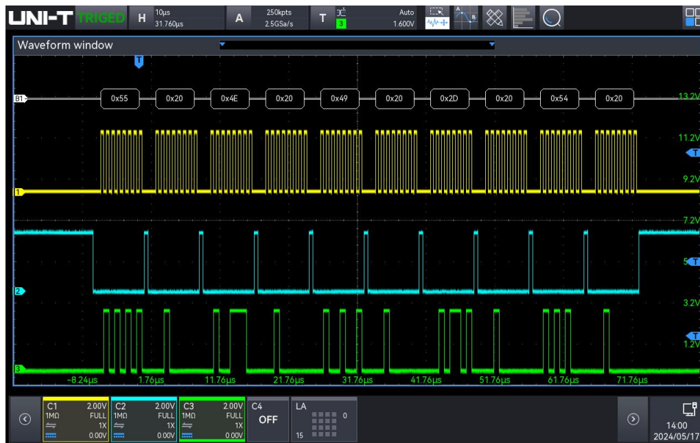
SPI trigger and decoding
