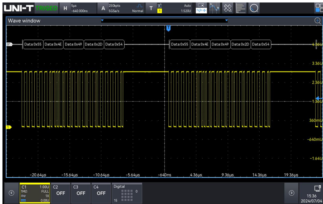
Manchester trigger and decoding
