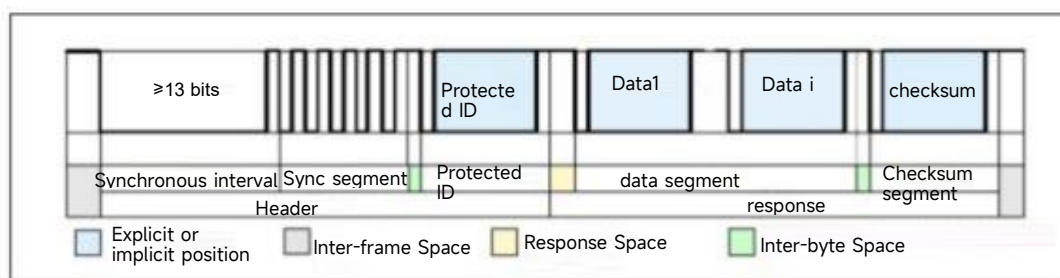
Frame structure
