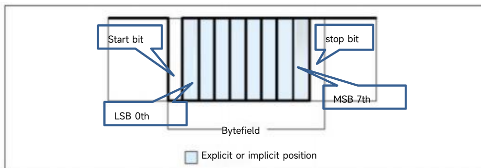
Frame structure
