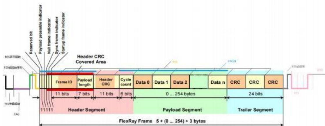
Figure 4-1: FlexRay frame format.
