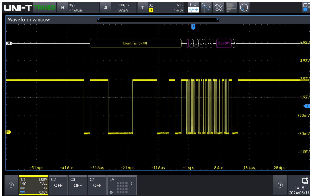
CAN-FD trigger and decoding
