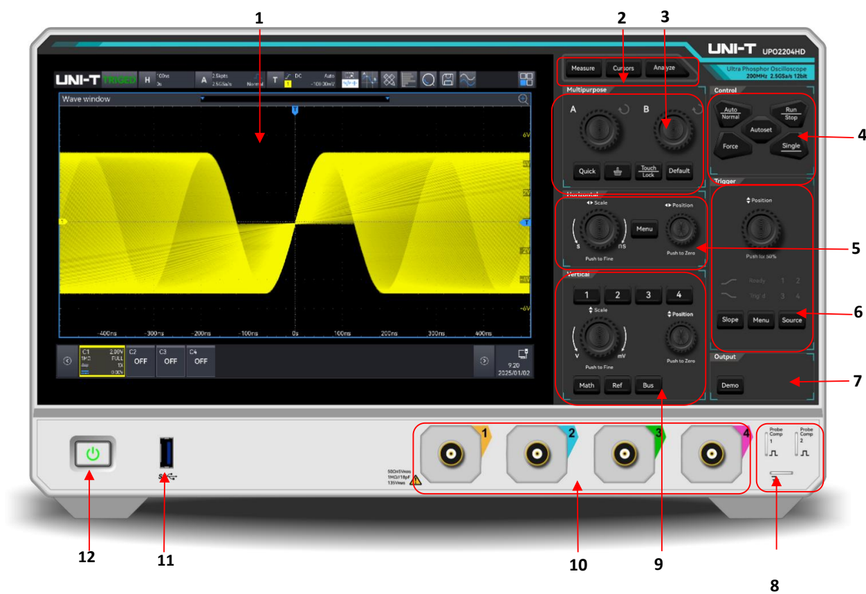
Front Panel
