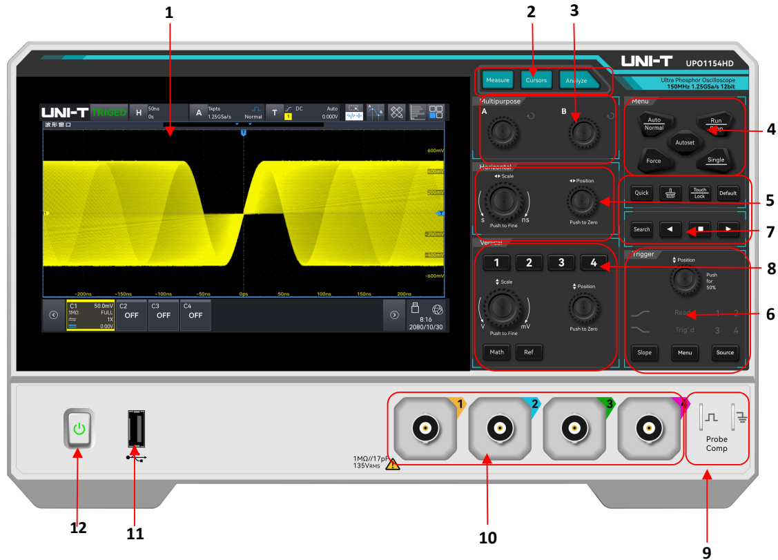
Front Panel
