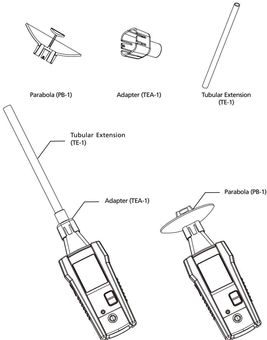
Figure 3.3: ULD-405 Accessories
