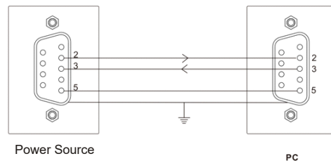
Rs232 Interface Definition
