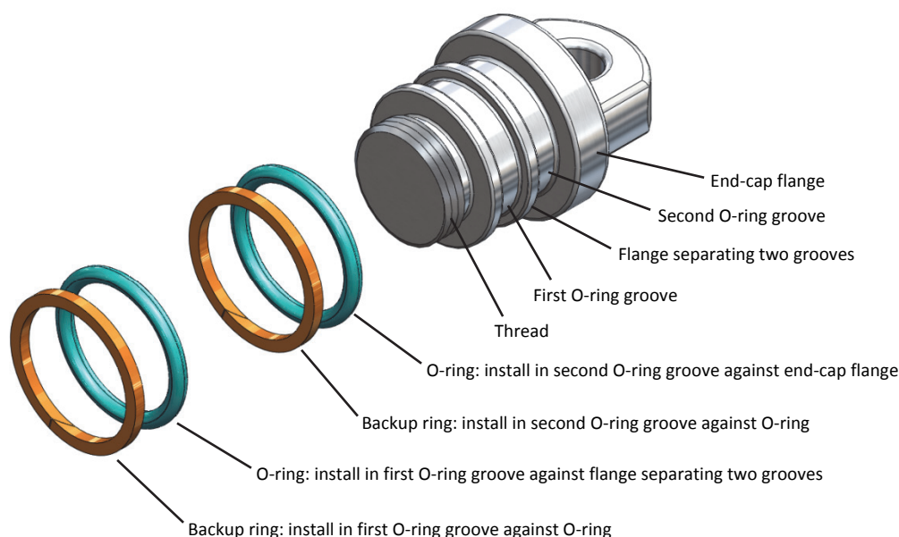
End-cap with the correct order of O-rings and backup rings
