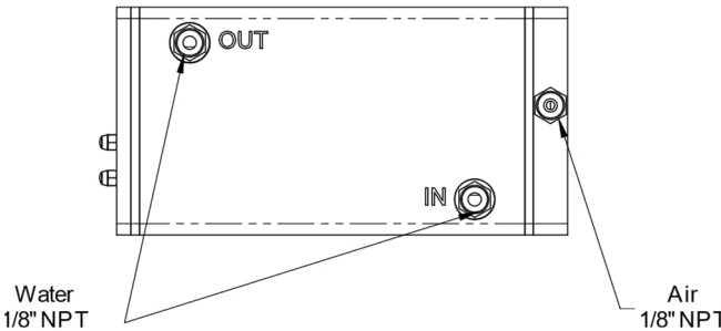
Figure 8-17: Enclosure Connections
