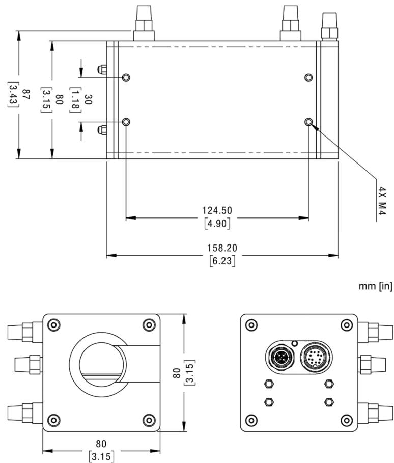
Figure 8-18: Enclosure Dimensions
