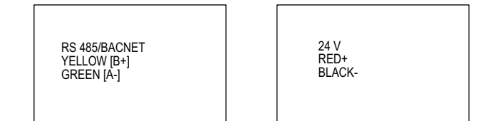
Figure 3: Cable labels
