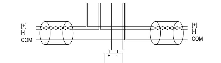
Figure 2: Local power supply
