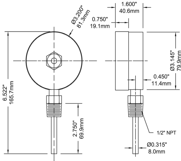
3" Bottom Connection
