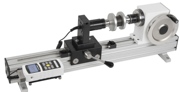
The TSTH is shown in a torsion spring test, with Series R50 torque sensor and Model M5i force/torque indicator
