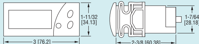
Panel Cutout 2-51/64" x 1-9/64" (71 x 29 mm)
