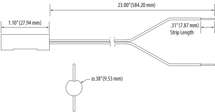
TRA Dimensional Drawing
