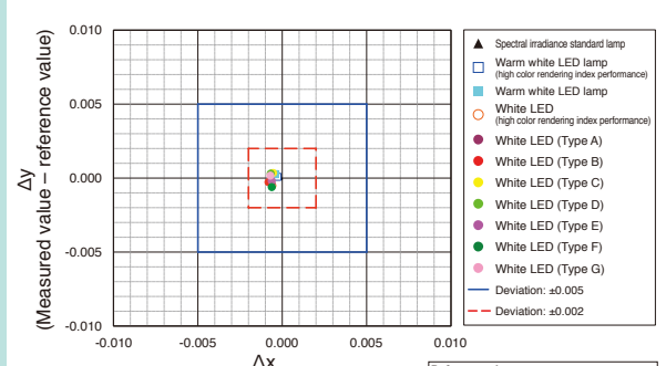
(Chromaticity measurement results for 10 types of white LED)
