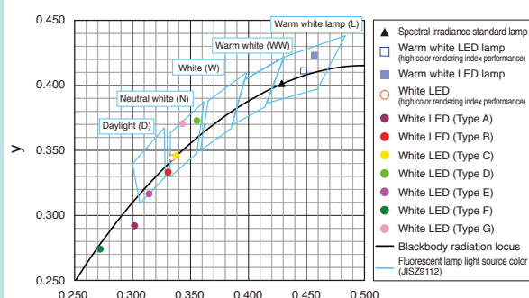
(Chromaticity measurement results for 10 types of white LED)
