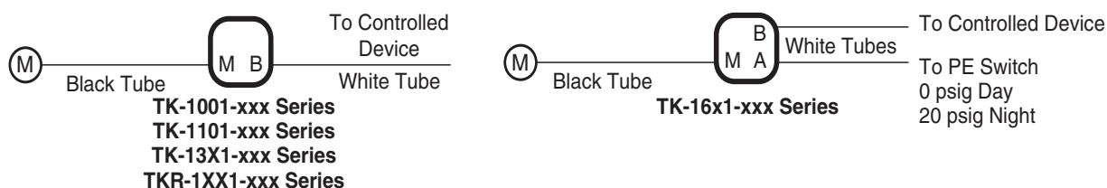
Figure 4 Two Pipe (Relay) Type.
