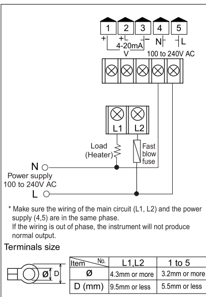
Main circuit
