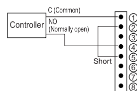
Contact input
