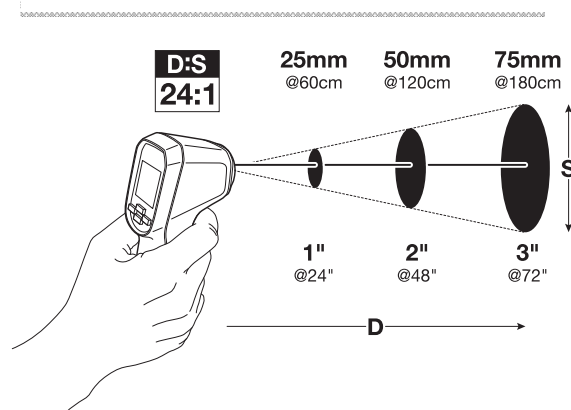
Fig 5-1 (a) TG54 Distance to Spot ratio 24:1
