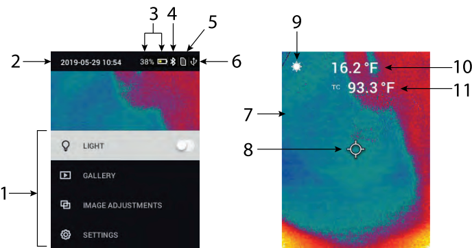
Figure 4.2 Display Description
