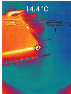
Figure 5.1 Combined Thermal and Visible Image (MSX®)
