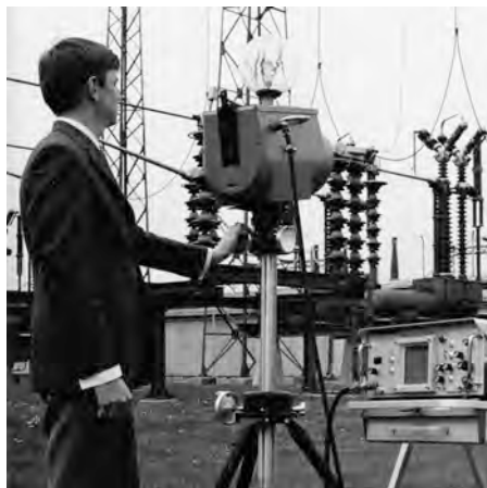
Figure 29.2 1969: Thermovision Model 661. The camera weighed approximately 25 kg (55 lb.), the oscilloscope 20 kg (44 lb.), and the tripod 15 kg (33 lb.). The operator also needed a 220 VAC generator set, and a 10 L (2.6 US gallon) jar with liquid nitrogen. To the left of the oscilloscope the Polaroid attachment (6 kg (13 lb.)) can be seen.
