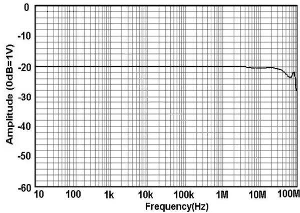
T3CP30-50 Frequency Response
