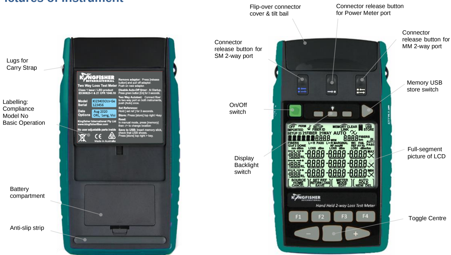
KI23400 / KI27400 HANDHELD 2-WAY LOSS TEST METER
