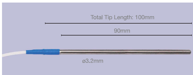
ST100L - Long Round Tip Probe
