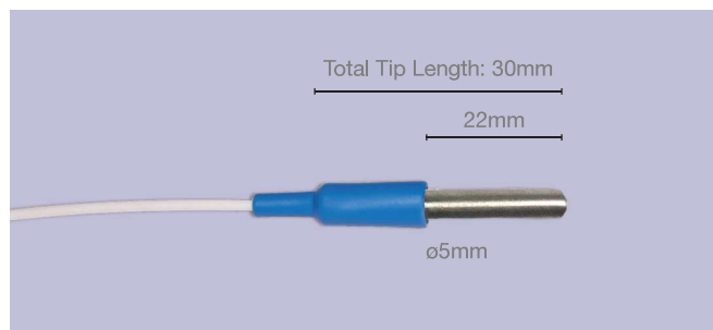
ST100S - Short Round Tip Sensor Probe
