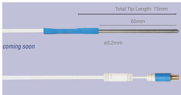
ST100KF - External Temperature Probe Flat Cable
