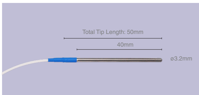
ST100J - Short Round Tip Probe
