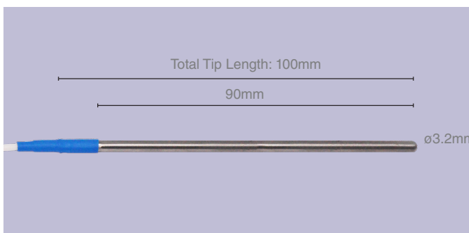
ST100L - Long Round Tip Probe
