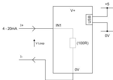
MEASURING 4-20mA USING A USB POWER SUPPLY
