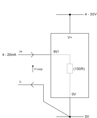
MEASURING 4-20mA
