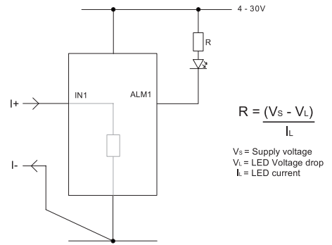
ALARM OUTPUT
