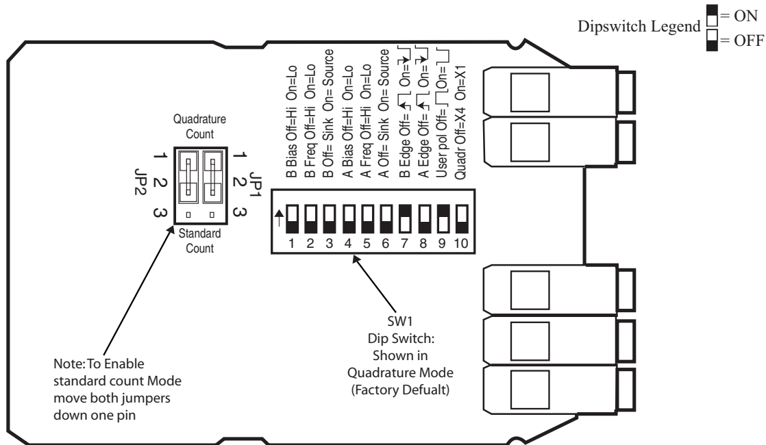
Figure 10. Quadrature Input Module Default Settings
