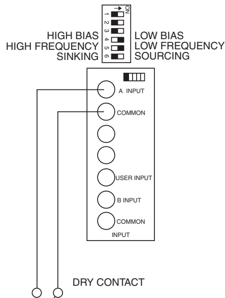
Figure 8a. Sensor Input example
