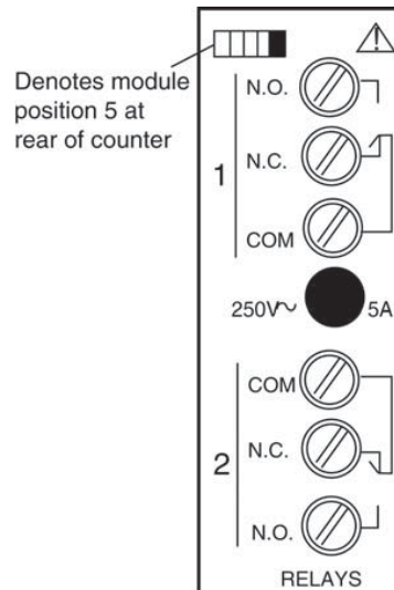
Figure 15. Dual Relay
