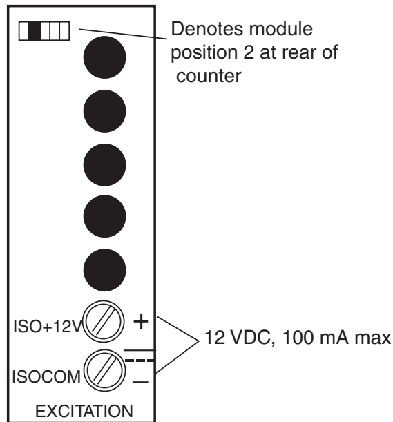
Figure 13. Excitation Module
