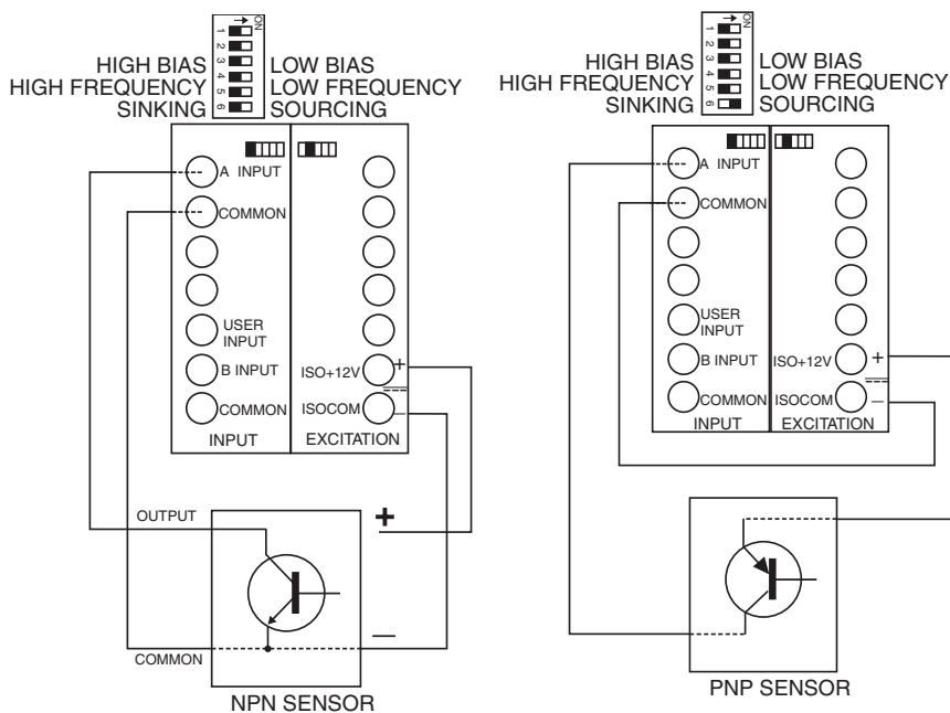
Figure 8. Sensor Connection Examples
