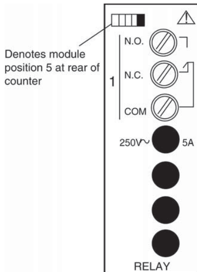
Figure 14. Single Relay
