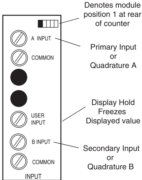
Figure 9. Quadrature / Universal Input Module
