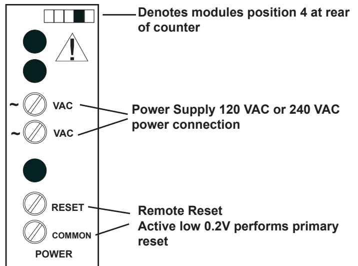
Figure 5. AC Power Module
