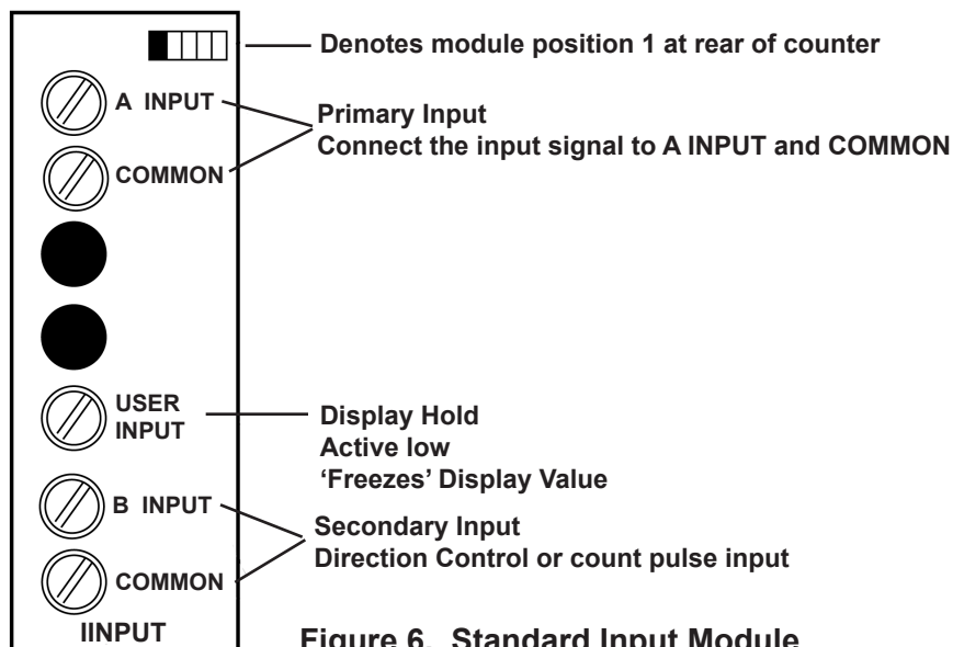
Figure 6. Standard Input Module
