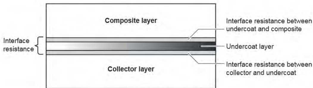
Figure: Diagram showing a cross-section of an electrode using a collector with an undercoat layer
