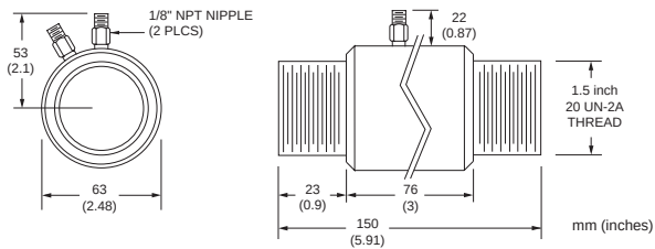
Figure B-8: GPS Head with Air /Water-cooled Housing
