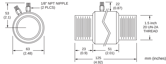
Figure B-7: GPR Head with Air /Water-cooled Housing
