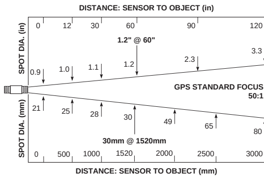
Figure B-14: GPS Standard Focus Optical Chart
