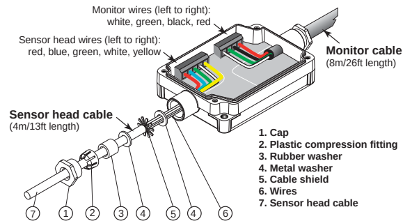
Figure B-4: Laser Switching Box Wiring Diagram
