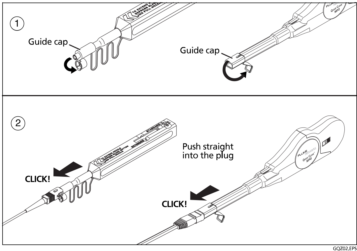
Figure 3. How to Clean Endfaces on Plugs
