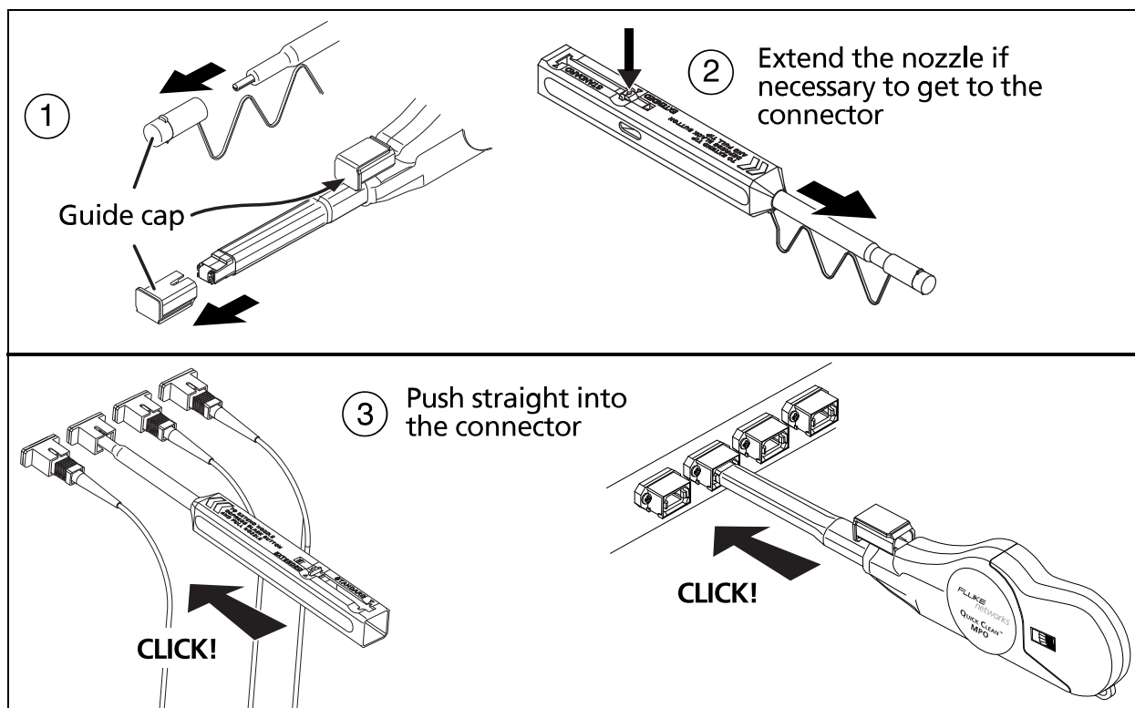
Figure 2. How to Clean Endfaces in Adapters
