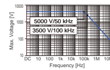
AC/DC HIGH VOLTAGE DIVIDER VT1005
