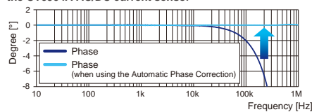
Example of the automatic phase correction for the CT6904A AC/DC current sensor
